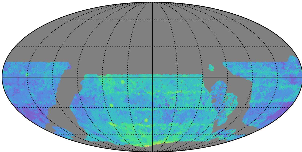
roll_pause_mjdp0_v3.4_10yrs WFD y band: Median Season Length
