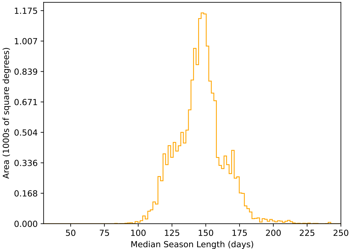
roll_pause_mjdp0_v3.4_10yrs WFD r band: Median Season Length
