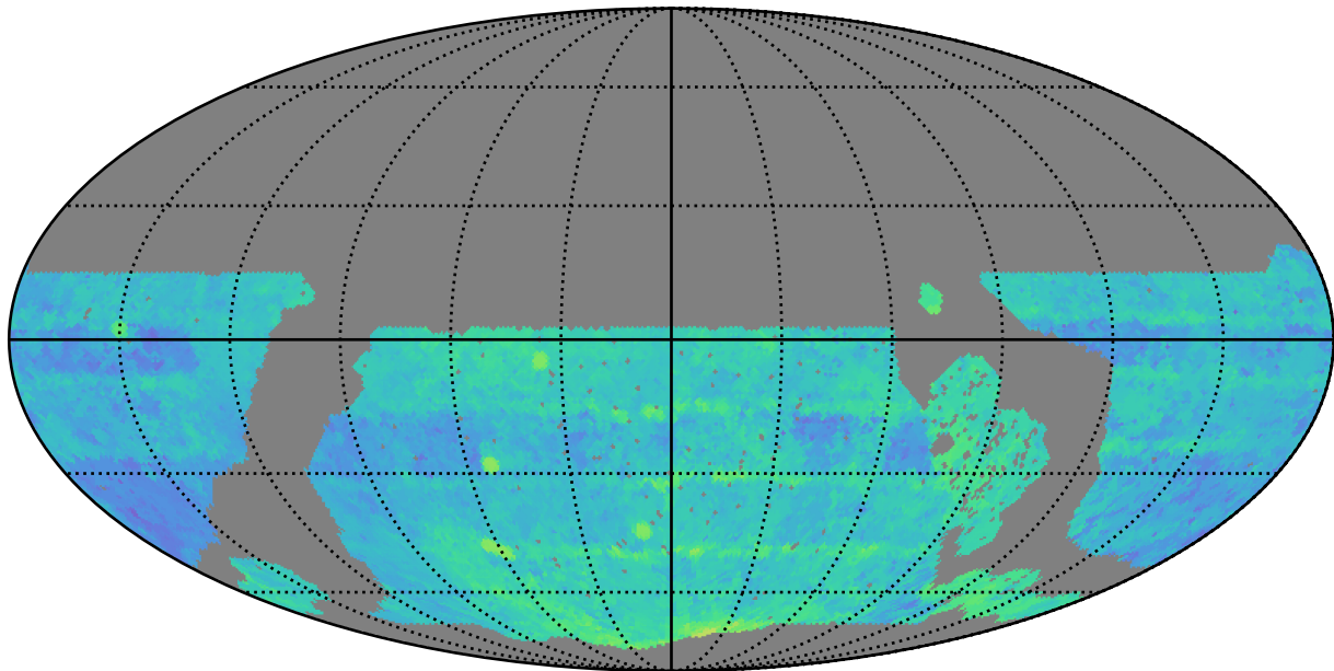
roll_pause_mjdp0_v3.4_10yrs WFD i band: Median Season Length
