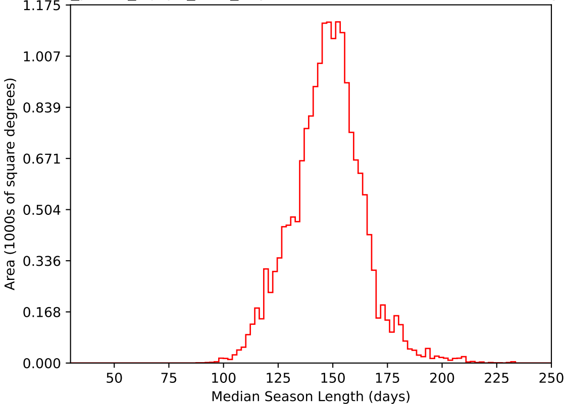
roll_pause_mjdp0_v3.4_10yrs WFD i band: Median Season Length
