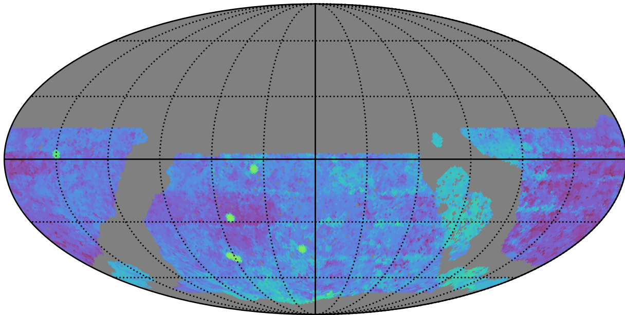
roll_pause_mjdp0_v3.4_10yrs WFD g band: Median Season Length
