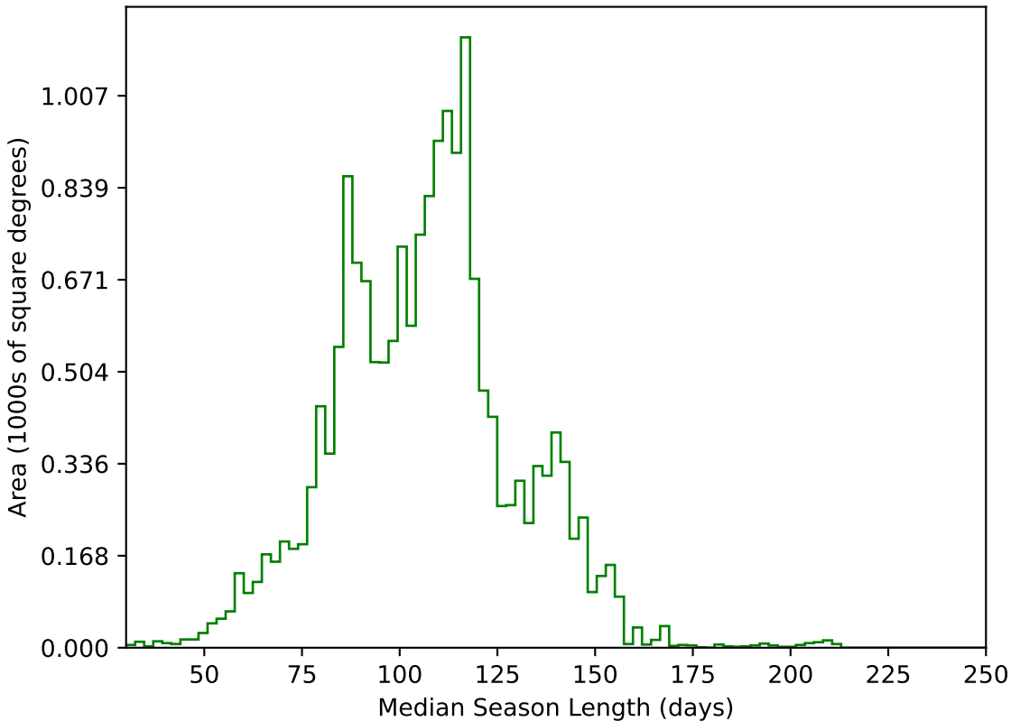
roll_pause_mjdp0_v3.4_10yrs WFD g band: Median Season Length
