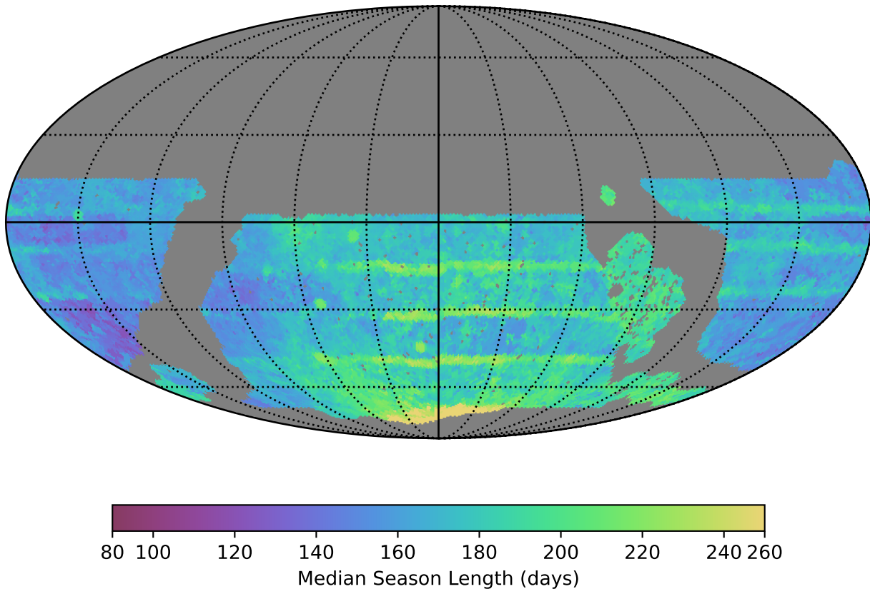
roll_pause_mjdp0_v3.4_10yrs WFD all bands: Median Season Length
