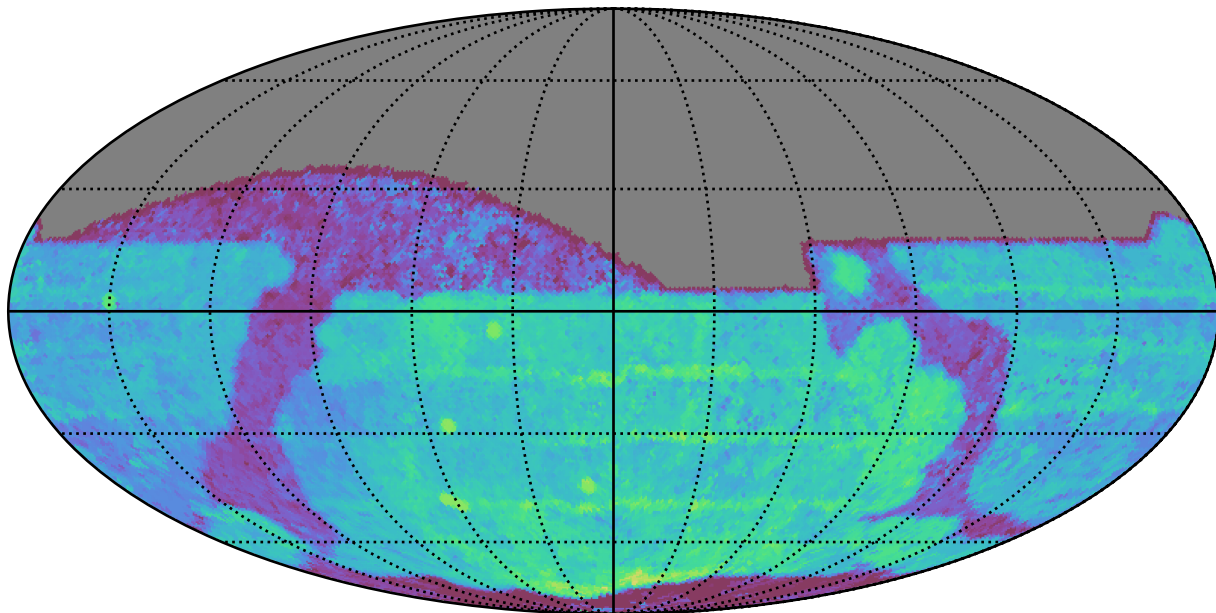
roll_pause_mjdp0_v3.4_10yrs All sky z band: Median Season Length
