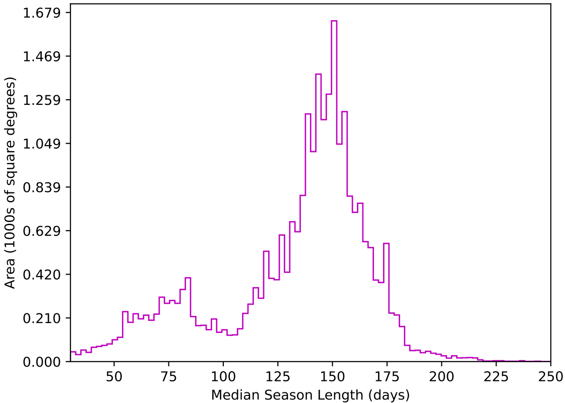
roll_pause_mjdp0_v3.4_10yrs All sky z band: Median Season Length
