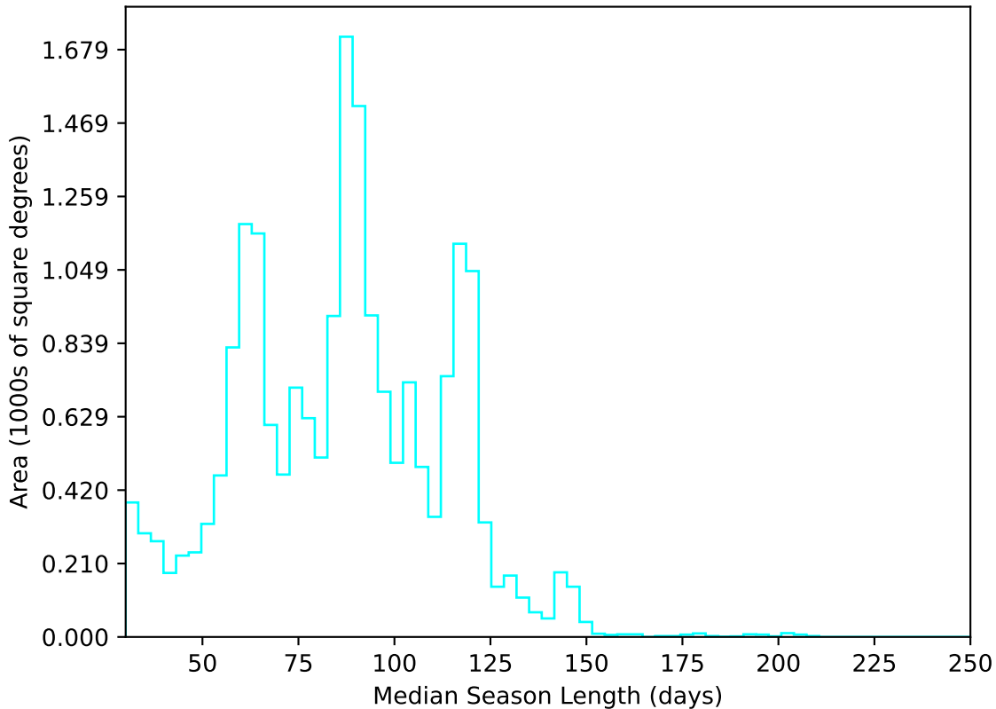
roll_pause_mjdp0_v3.4_10yrs All sky u band: Median Season Length
