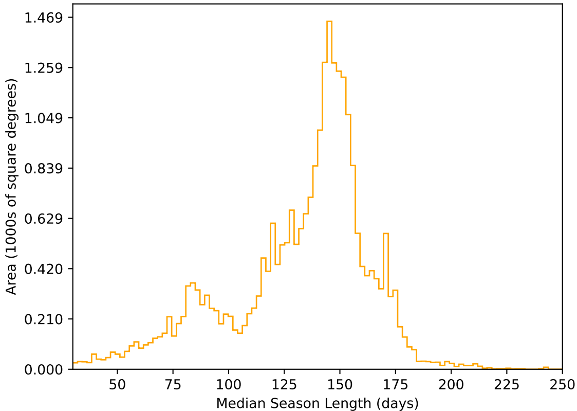
roll_pause_mjdp0_v3.4_10yrs All sky r band: Median Season Length
