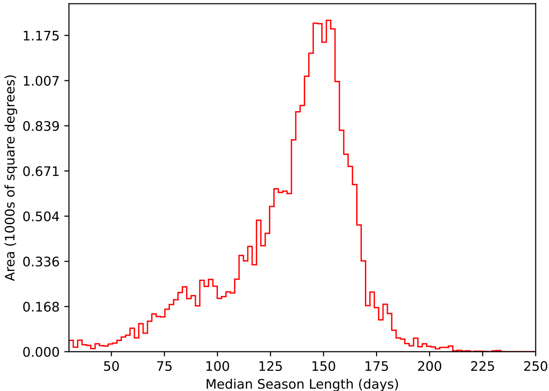
roll_pause_mjdp0_v3.4_10yrs All sky i band: Median Season Length
