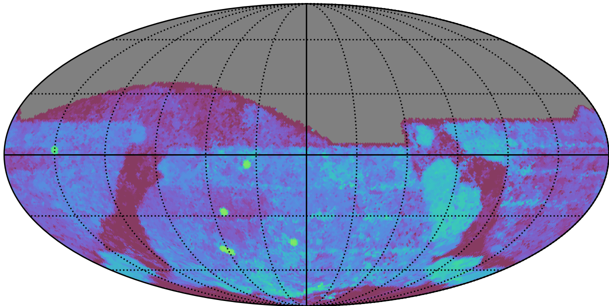
roll_pause_mjdp0_v3.4_10yrs All sky g band: Median Season Length
