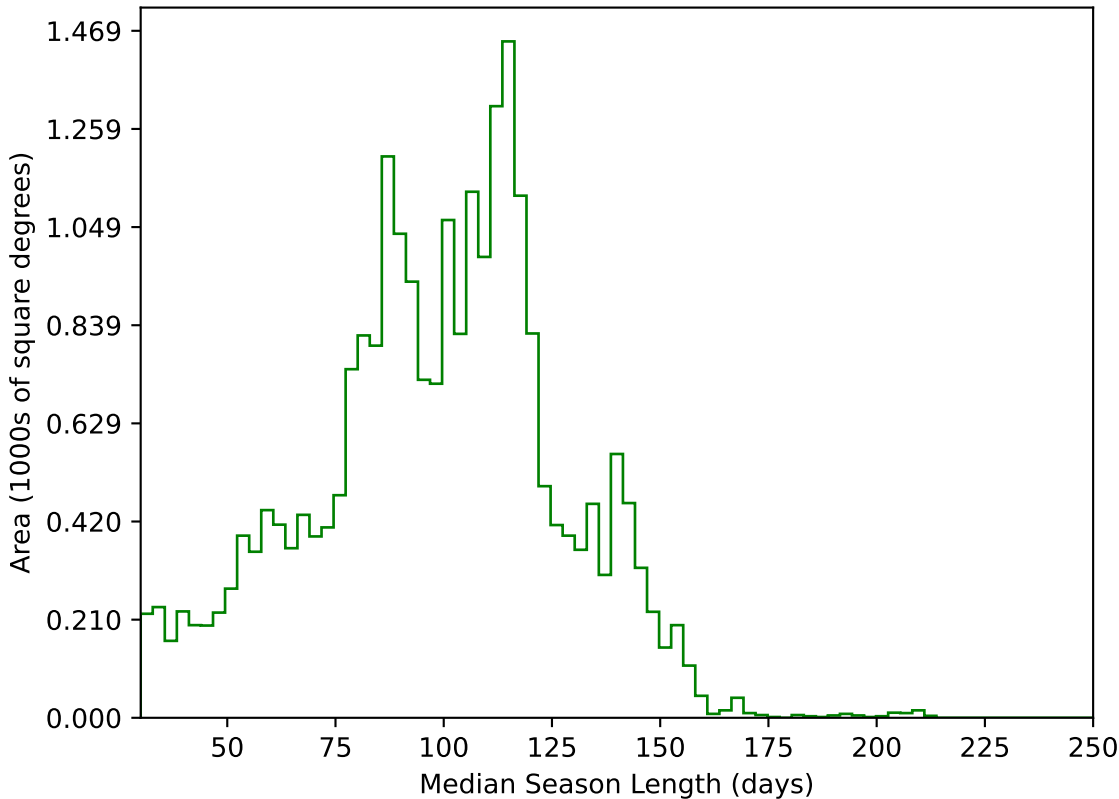
roll_pause_mjdp0_v3.4_10yrs All sky g band: Median Season Length
