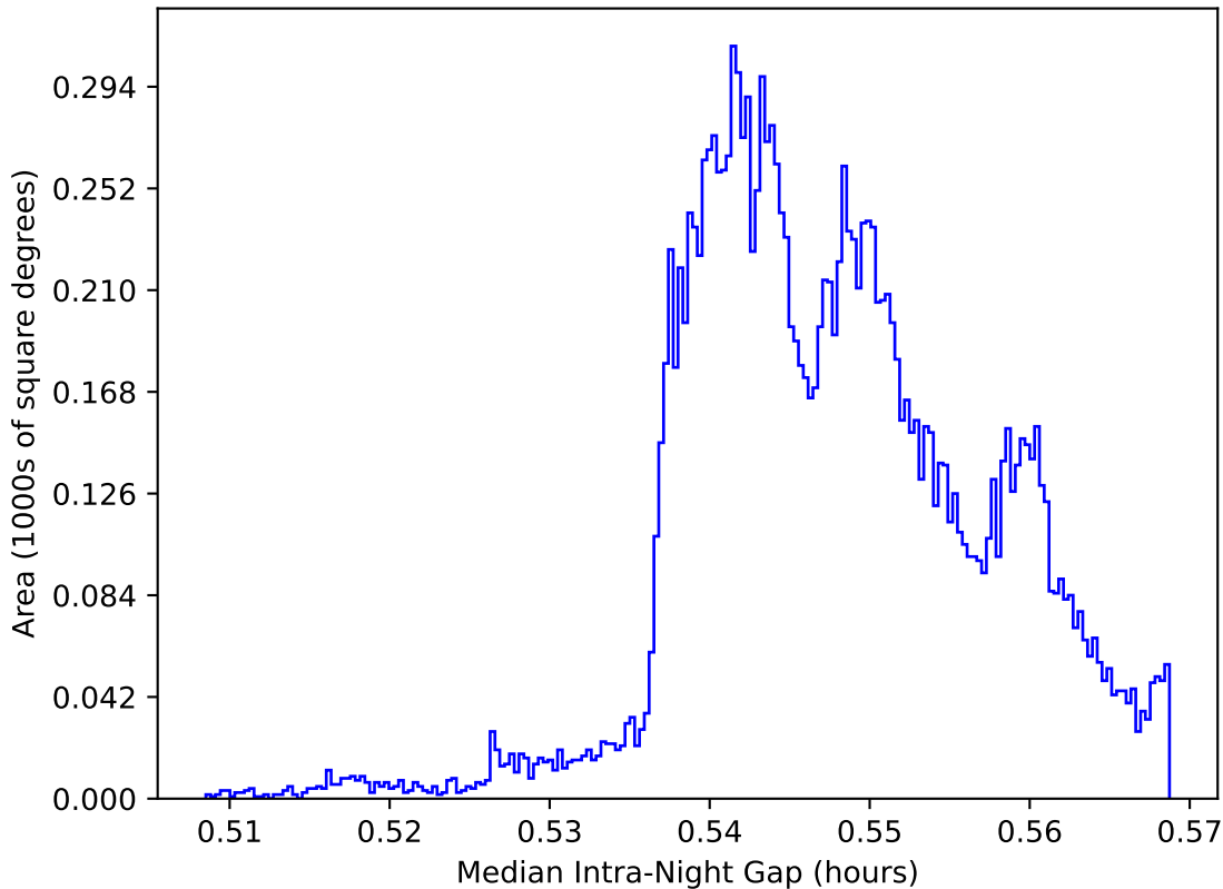
roll_pause_mjdp0_v3.4_10yrs WFD: Median Intra-Night Gap
