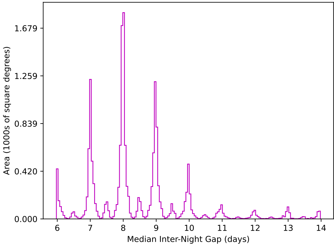
roll_pause_mjdp0_v3.4_10yrs WFD z band: Median Inter-Night Gap
