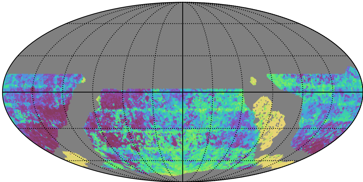
roll_pause_mjdp0_v3.4_10yrs WFD y band: Median Inter-Night Gap
