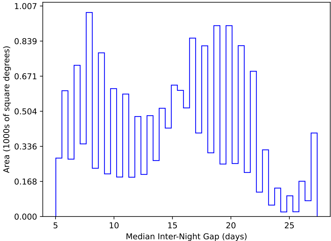
roll_pause_mjdp0_v3.4_10yrs WFD y band: Median Inter-Night Gap
