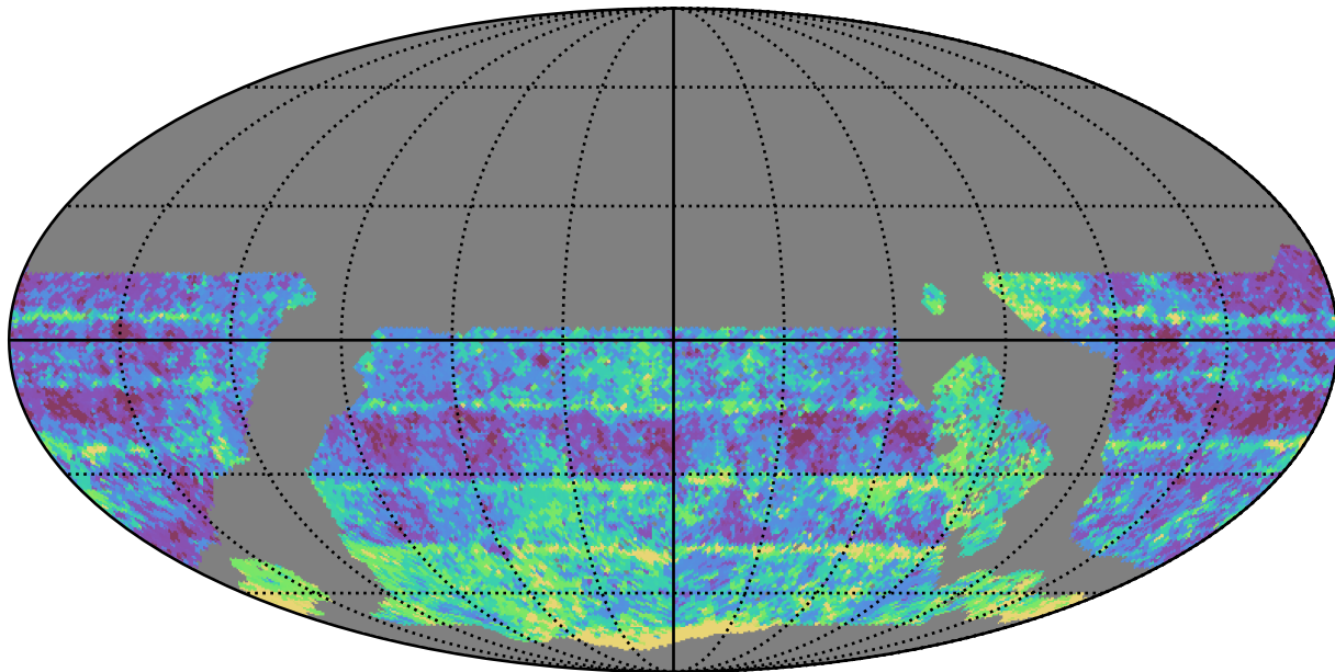
roll_pause_mjdp0_v3.4_10yrs WFD r band: Median Inter-Night Gap
