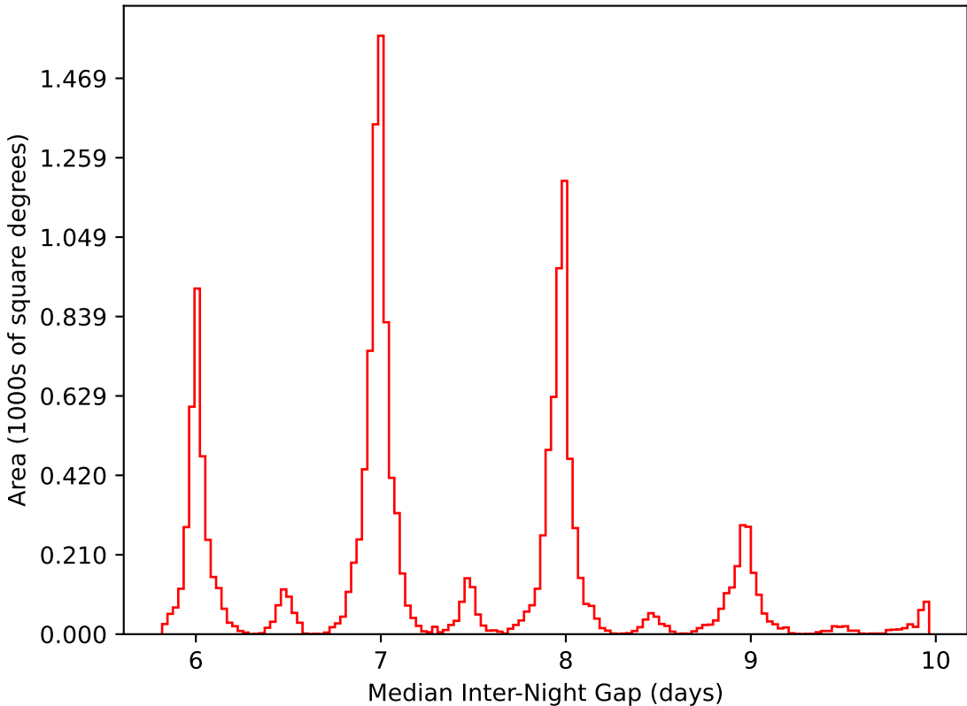
roll_pause_mjdp0_v3.4_10yrs WFD i band: Median Inter-Night Gap
