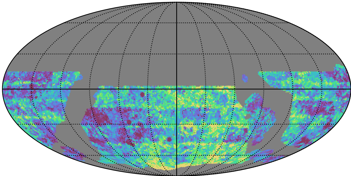
roll_pause_mjdp0_v3.4_10yrs WFD g band: Median Inter-Night Gap
