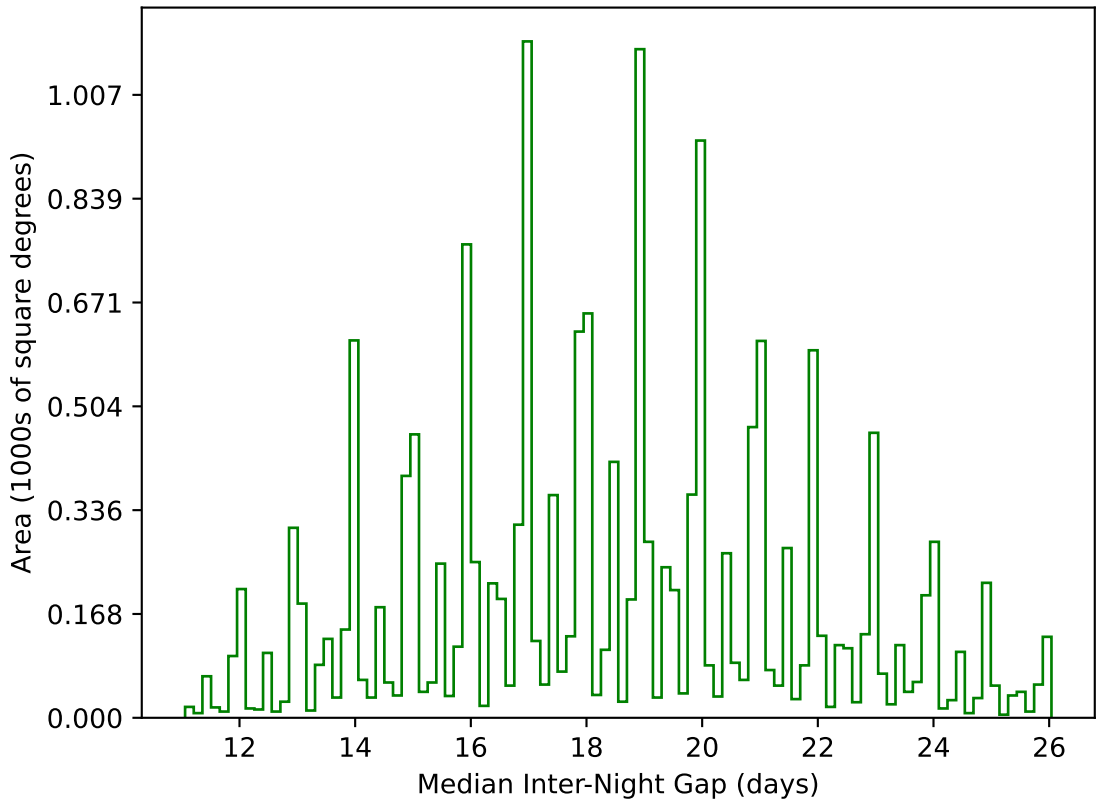
roll_pause_mjdp0_v3.4_10yrs WFD g band: Median Inter-Night Gap
