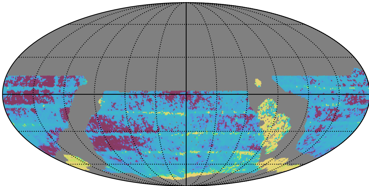
roll_pause_mjdp0_v3.4_10yrs WFD all bands: Median Inter-Night Gap
