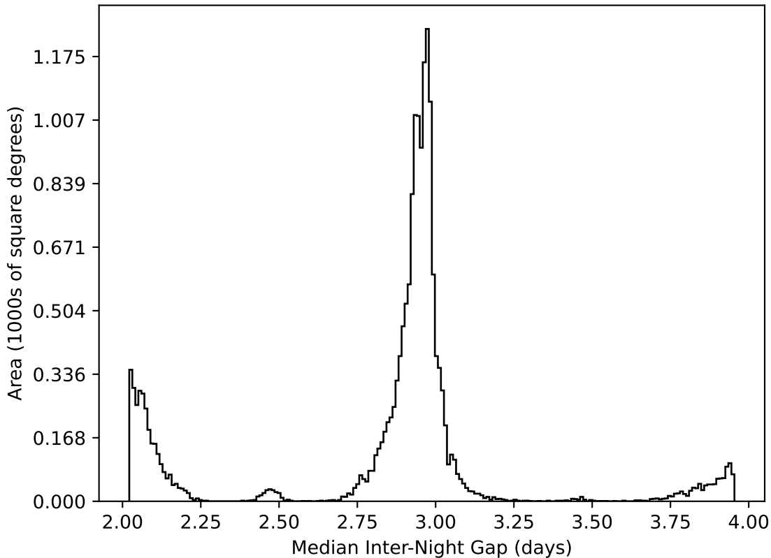
roll_pause_mjdp0_v3.4_10yrs WFD all bands: Median Inter-Night Gap
