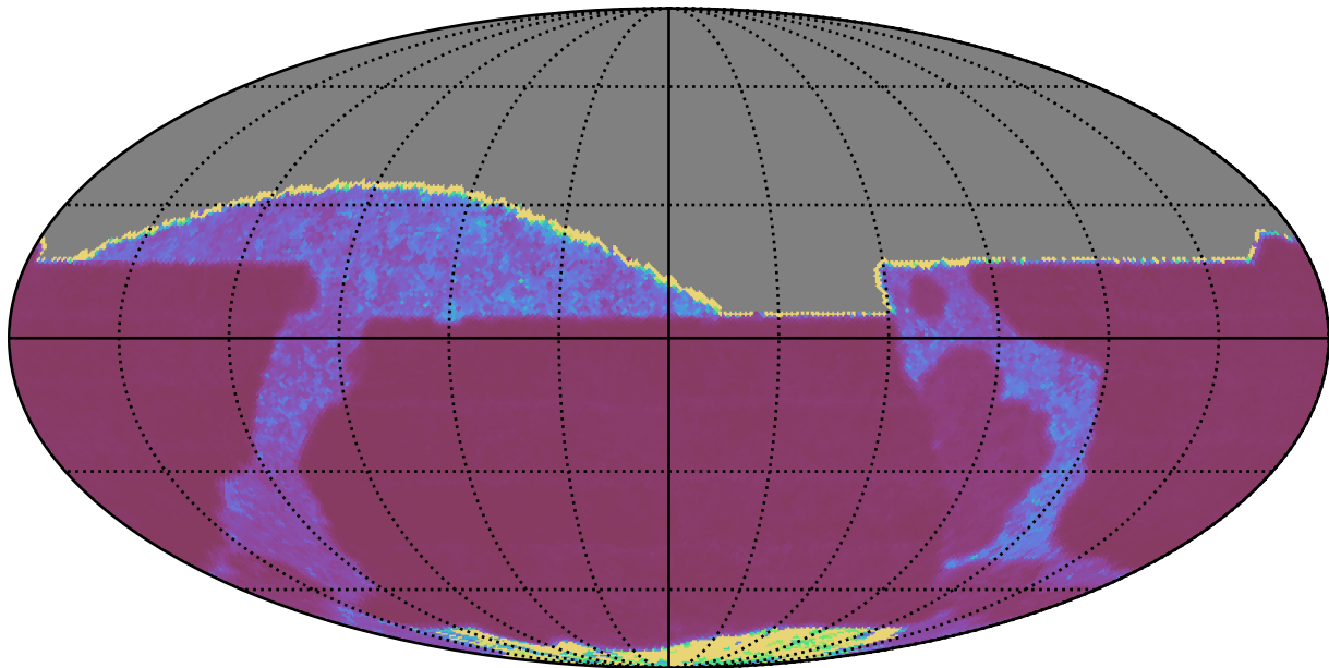
roll_pause_mjdp0_v3.4_10yrs All sky z band: Median Inter-Night Gap
