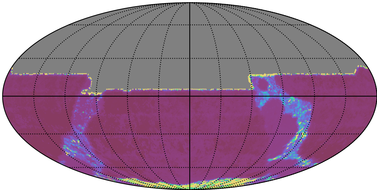
roll_pause_mjdp0_v3.4_10yrs All sky y band: Median Inter-Night Gap
