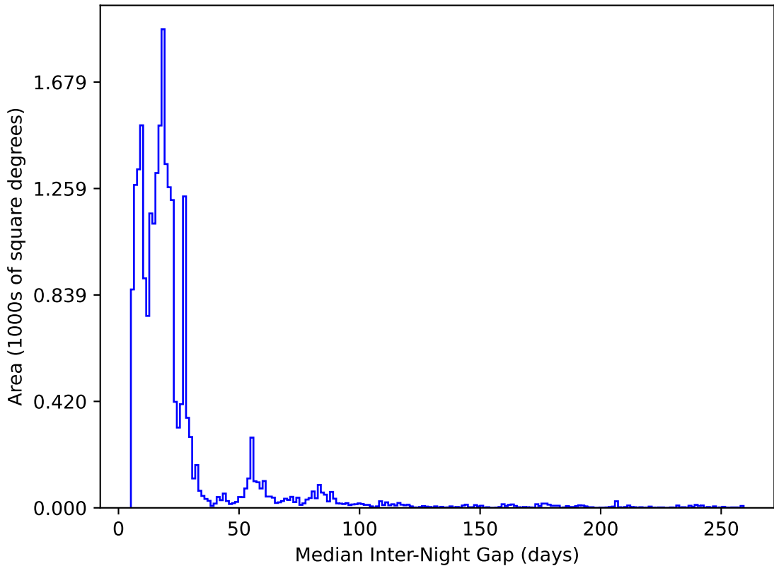
roll_pause_mjdp0_v3.4_10yrs All sky y band: Median Inter-Night Gap
