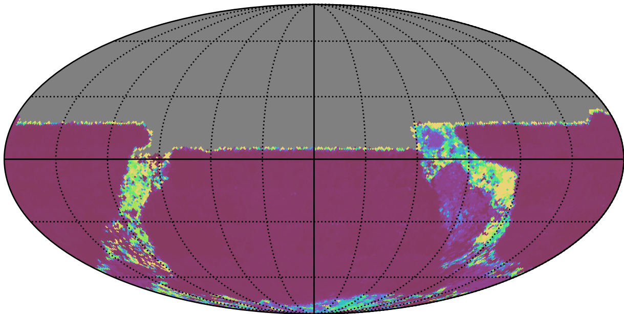
roll_pause_mjdp0_v3.4_10yrs All sky u band: Median Inter-Night Gap
