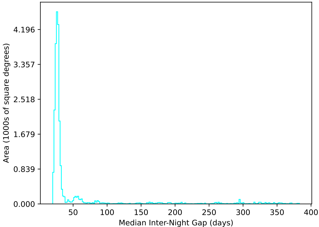
roll_pause_mjdp0_v3.4_10yrs All sky u band: Median Inter-Night Gap
