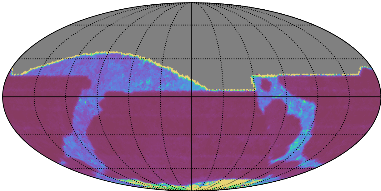
roll_pause_mjdp0_v3.4_10yrs All sky r band: Median Inter-Night Gap
