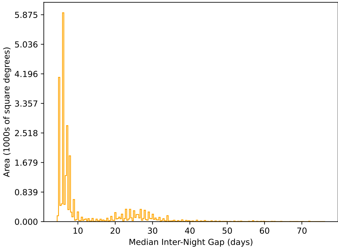
roll_pause_mjdp0_v3.4_10yrs All sky r band: Median Inter-Night Gap
