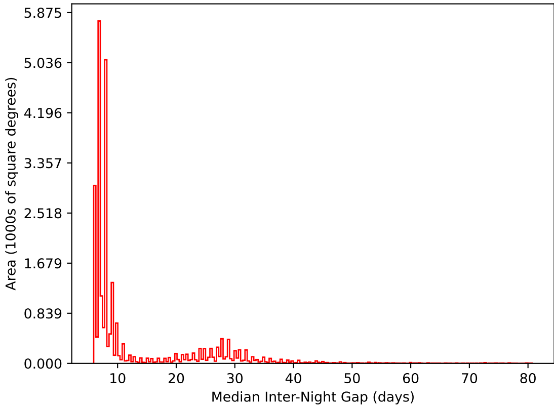
roll_pause_mjdp0_v3.4_10yrs All sky i band: Median Inter-Night Gap
