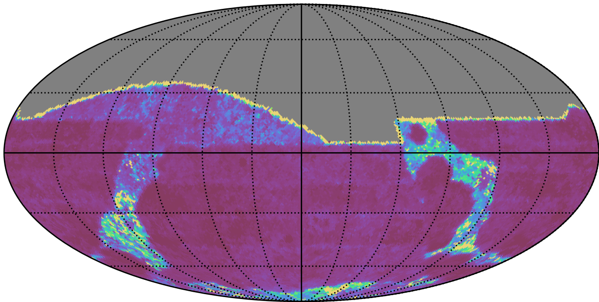
roll_pause_mjdp0_v3.4_10yrs All sky g band: Median Inter-Night Gap
