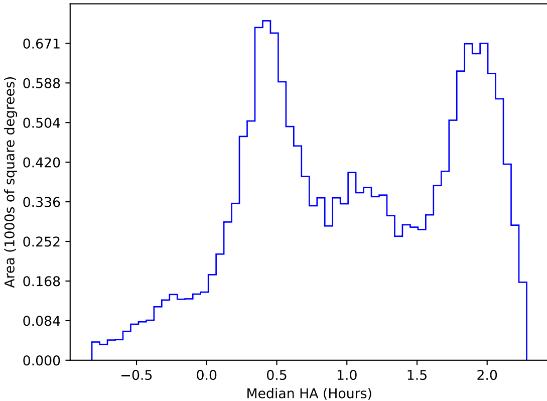
roll_pause_mjdp0_v3.4_10yrs WFD z band: Median HA
