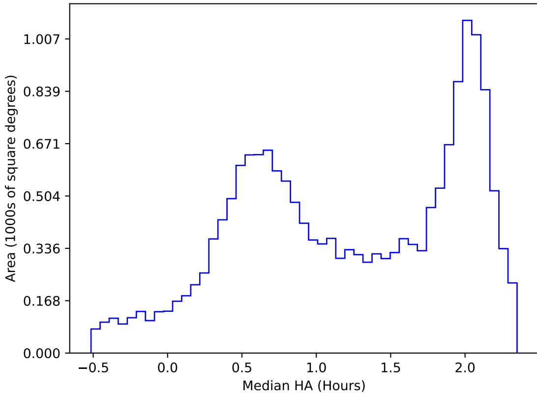
roll_pause_mjdp0_v3.4_10yrs WFD y band: Median HA
