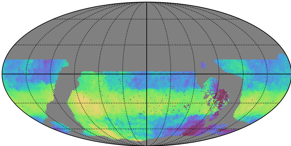
roll_pause_mjdp0_v3.4_10yrs WFD u band: Median HA
