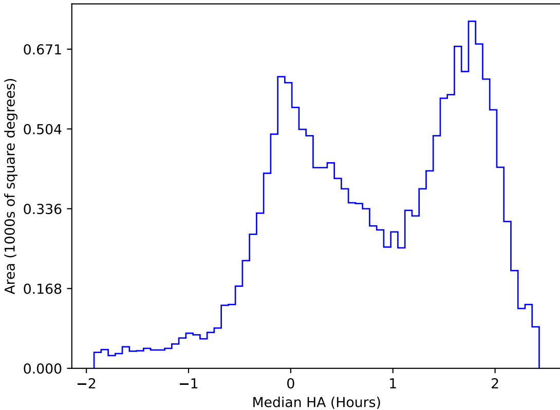
roll_pause_mjdp0_v3.4_10yrs WFD u band: Median HA
