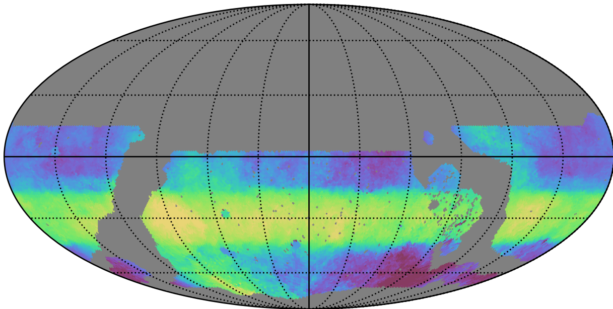
roll_pause_mjdp0_v3.4_10yrs WFD r band: Median HA
