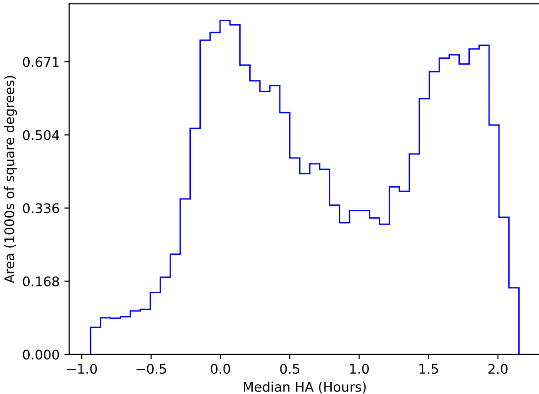
roll_pause_mjdp0_v3.4_10yrs WFD r band: Median HA
