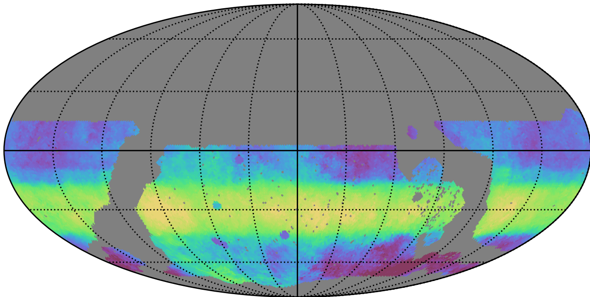
roll_pause_mjdp0_v3.4_10yrs WFD i band: Median HA
