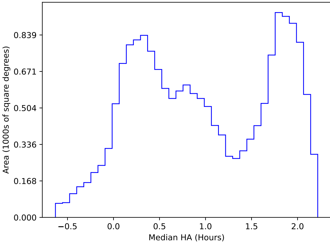
roll_pause_mjdp0_v3.4_10yrs WFD i band: Median HA
