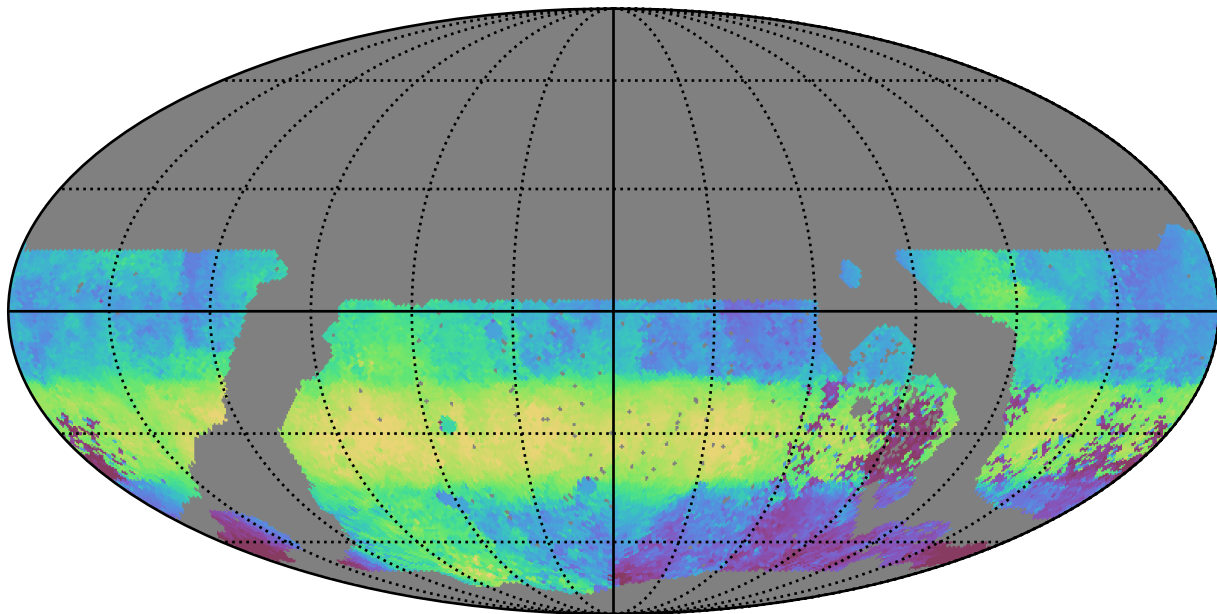
roll_pause_mjdp0_v3.4_10yrs WFD g band: Median HA
