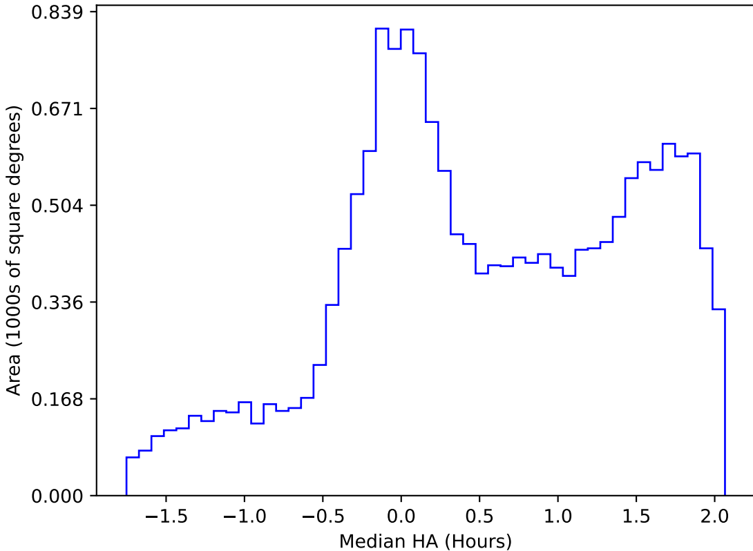
roll_pause_mjdp0_v3.4_10yrs WFD g band: Median HA
