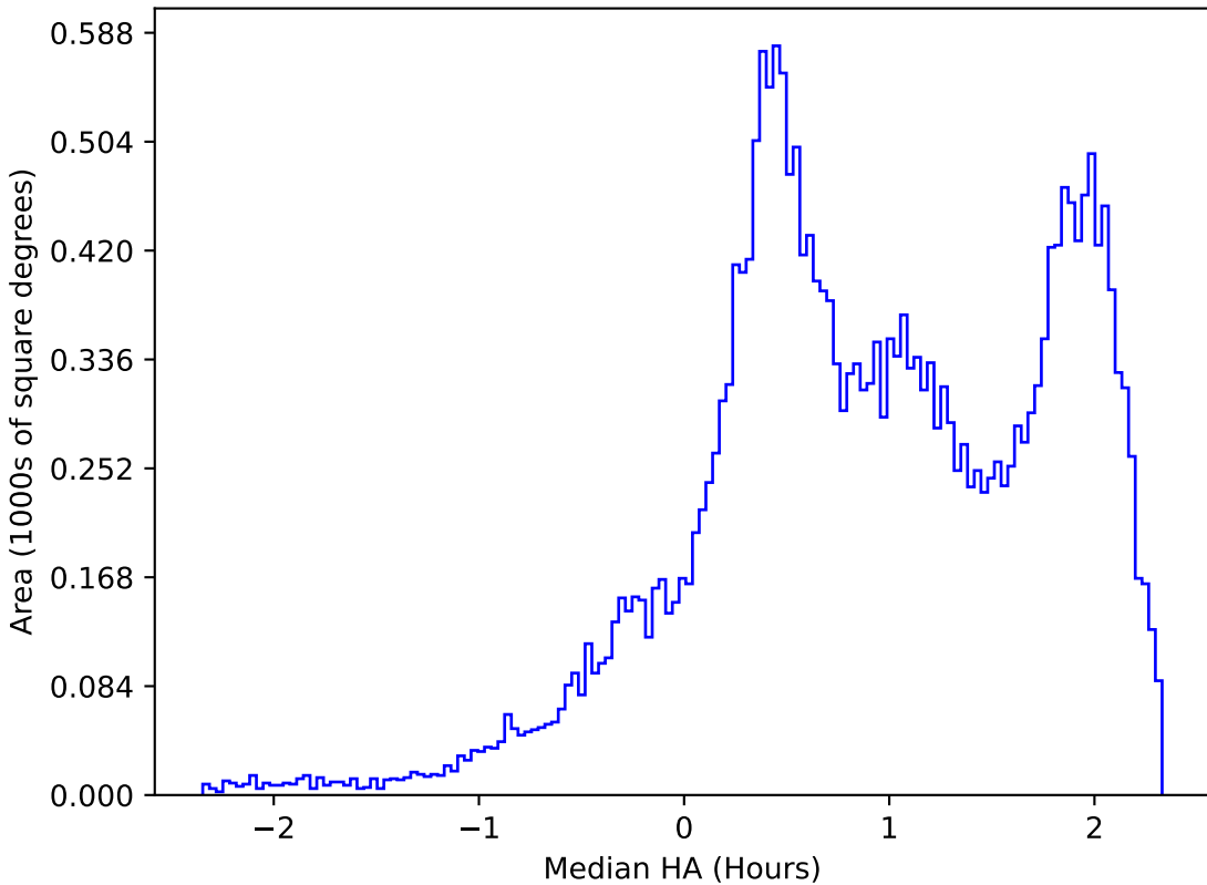
roll_pause_mjdp0_v3.4_10yrs All sky z band: Median HA
