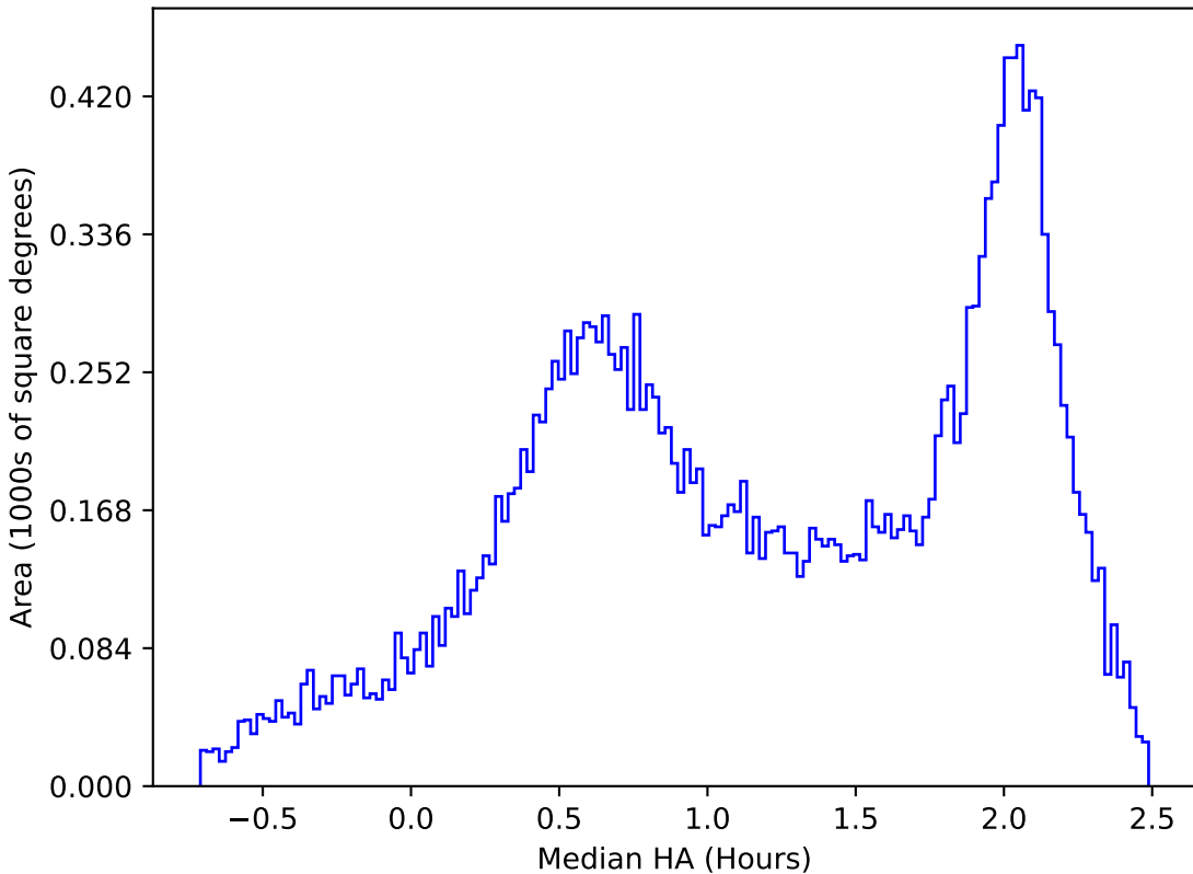
roll_pause_mjdp0_v3.4_10yrs All sky y band: Median HA
