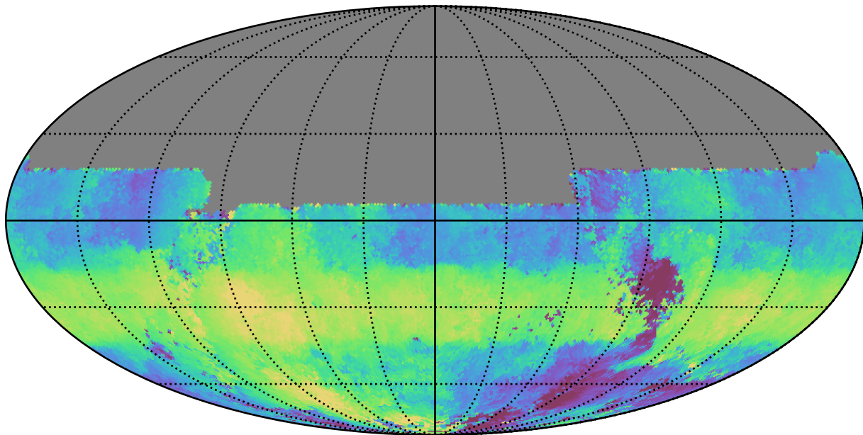
roll_pause_mjdp0_v3.4_10yrs All sky u band: Median HA
