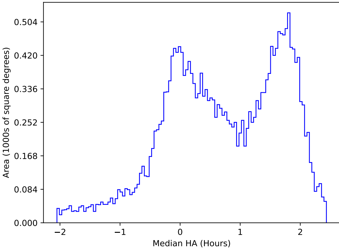
roll_pause_mjdp0_v3.4_10yrs All sky u band: Median HA
