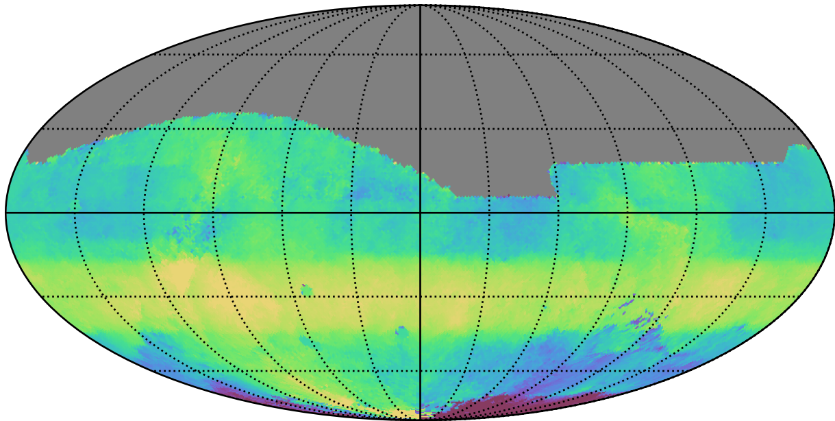
roll_pause_mjdp0_v3.4_10yrs All sky r band: Median HA
