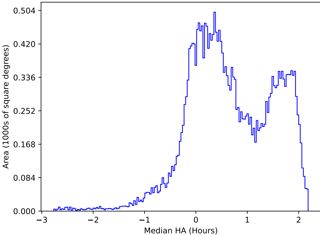
roll_pause_mjdp0_v3.4_10yrs All sky r band: Median HA
