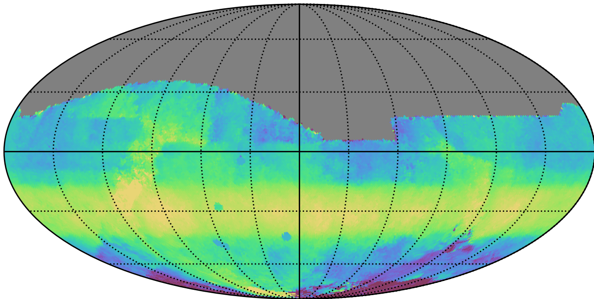
roll_pause_mjdp0_v3.4_10yrs All sky i band: Median HA
